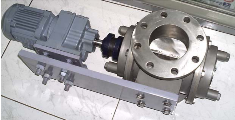
SIZE 6.0" ,SUS 304, with water cooling chamber ,for car coolant film scrap recycle, pneumatic conveying system
